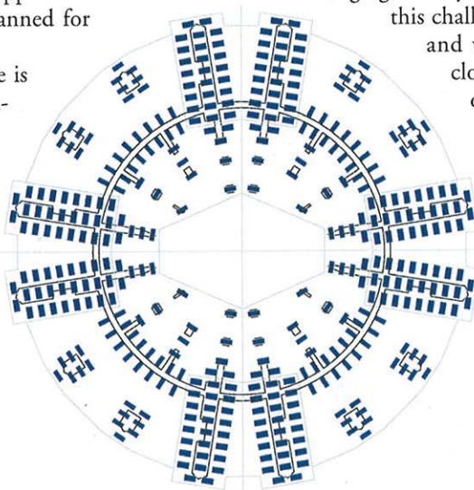
Foundation Barrette Plan.
